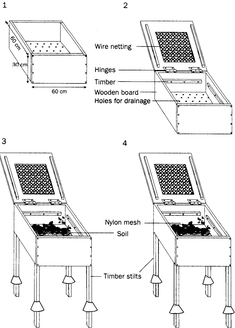
Figure 9: Sequence of building a single chamber hutch box
